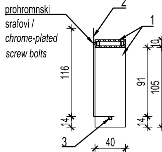
Presek 1-1 / Section 1-1
