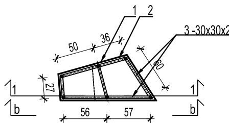
Presek 2-2/ Section 2-2
