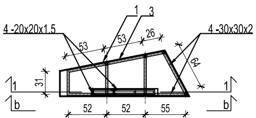
Presek 2-2/ Section 2-2
