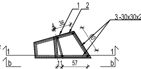
Presek 3-3 / Section 3-3
