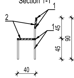
Presek 1-1 / Section 1-1
