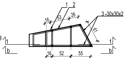
Presek 3-3 / Section 3-3
