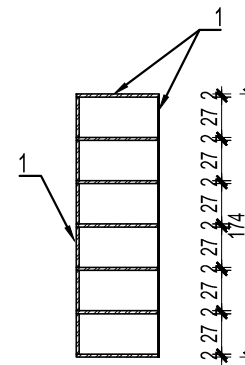
Presek 1-1 / Section 1-1
