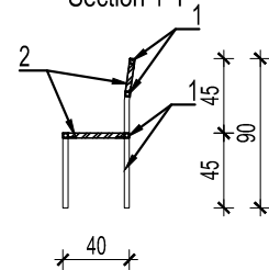
Presek 1-1 / Section 1-1
