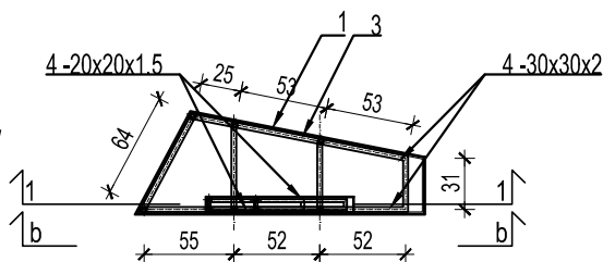
Presek 2-2/ Section 2-2
