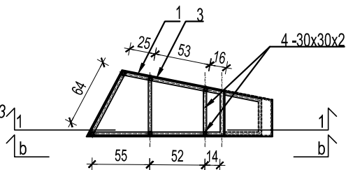
Presek 3-3 / Section 3-3
