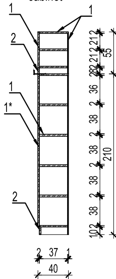
Presek 1-1 / Section 1-1
